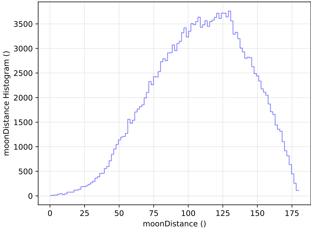
too_elab_r16_d3_ugrizy_v3.4_10yrs WFD g band: moonDistance Histogram
