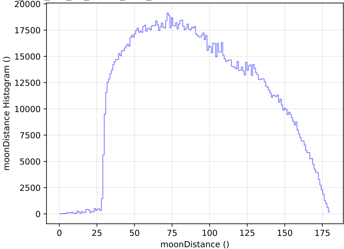
too_elab_r16_d3_ugrizy_v3.4_10yrs WFD all bands: moonDistance Histogram
