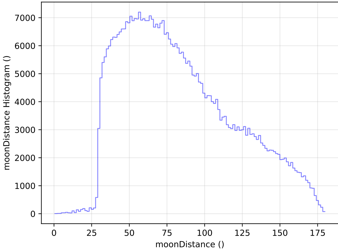
too_elab_r16_d3_ugrizy_v3.4_10yrs All sky z band: moonDistance Histogram
