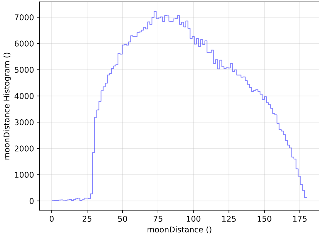
too_elab_r16_d3_ugrizy_v3.4_10yrs All sky i band: moonDistance Histogram
