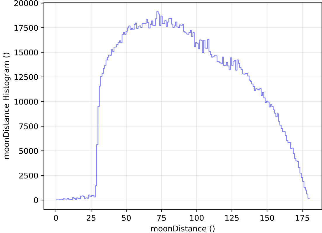
too_elab_r16_d3_ugrizy_v3.4_10yrs All sky all bands: moonDistance Histogram
