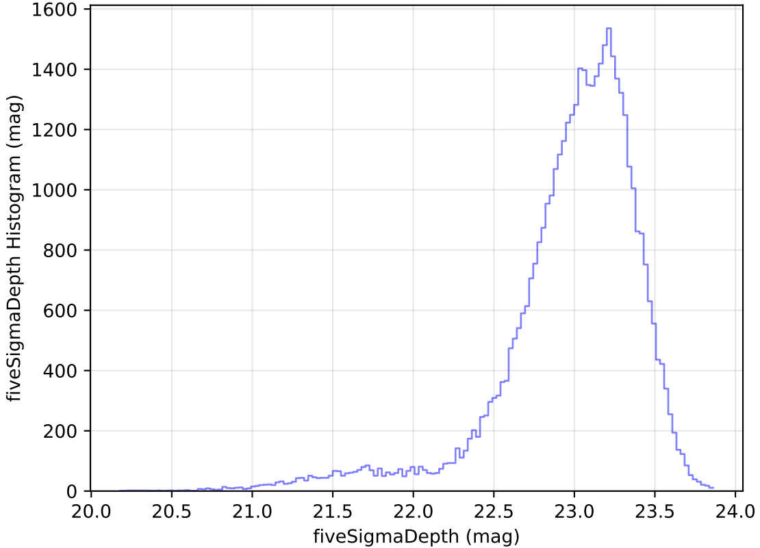
too_elab_r16_d3_ugrizy_v3.4_10yrs Yr 1 z band: fiveSigmaDepth Histogram
