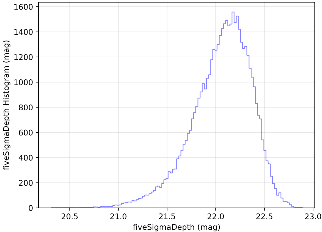
too_elab_r16_d3_ugrizy_v3.4_10yrs Yr 1 y band: fiveSigmaDepth Histogram
