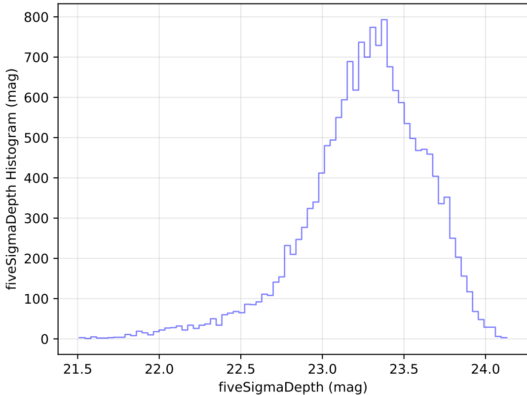
too_elab_r16_d3_ugrizy_v3.4_10yrs Yr 1 u band: fiveSigmaDepth Histogram
