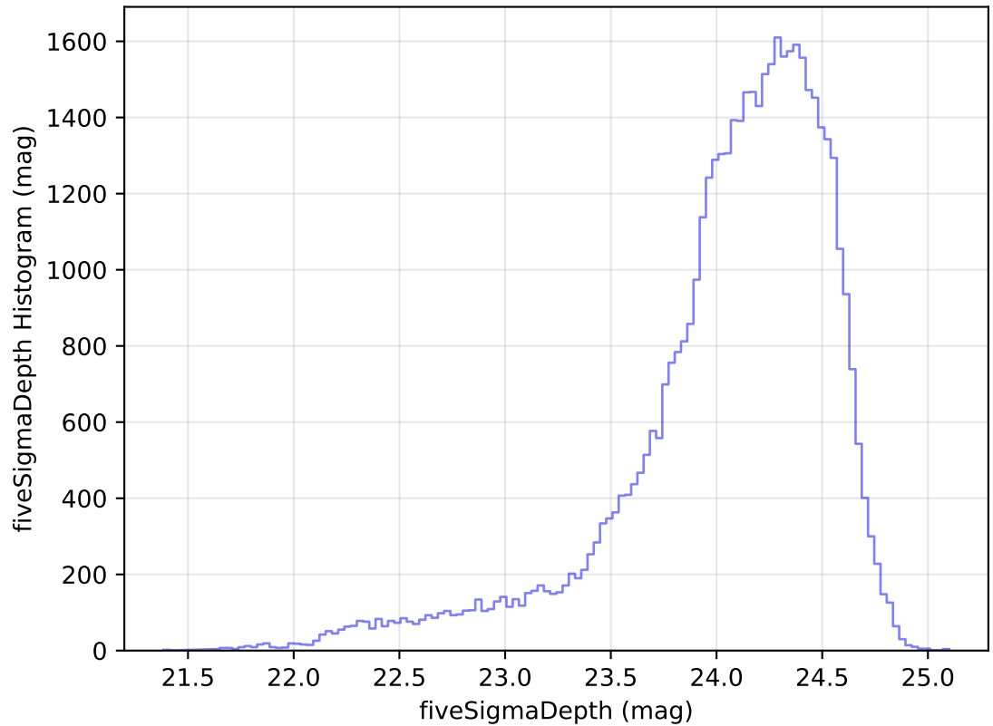
too_elab_r16_d3_ugrizy_v3.4_10yrs Yr 1 r band: fiveSigmaDepth Histogram
