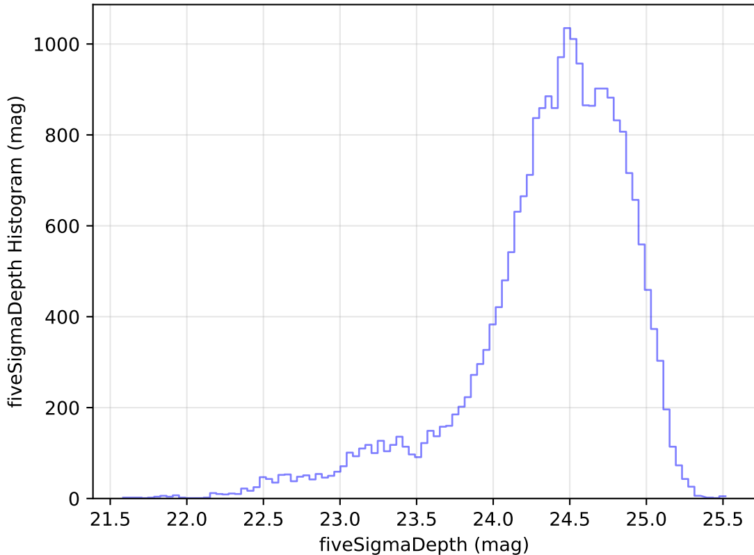
too_elab_r16_d3_ugrizy_v3.4_10yrs Yr 1 g band: fiveSigmaDepth Histogram
