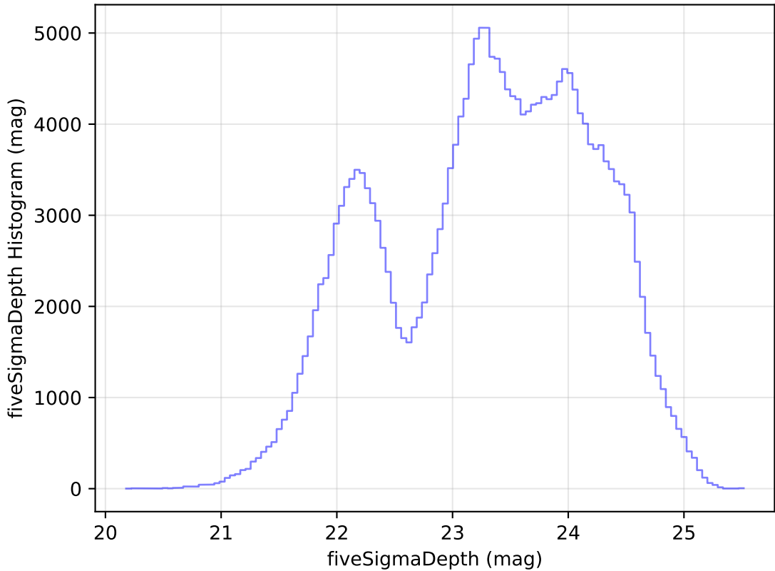
too_elab_r16_d3_ugrizy_v3.4_10yrs Yr 1 all bands: fiveSigmaDepth Histogram
