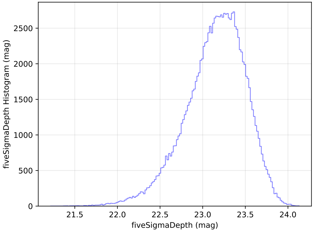
too_elab_r16_d3_ugrizy_v3.4_10yrs WFD u band: fiveSigmaDepth Histogram
