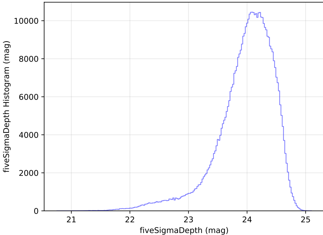
too_elab_r16_d3_ugrizy_v3.4_10yrs WFD r band: fiveSigmaDepth Histogram
