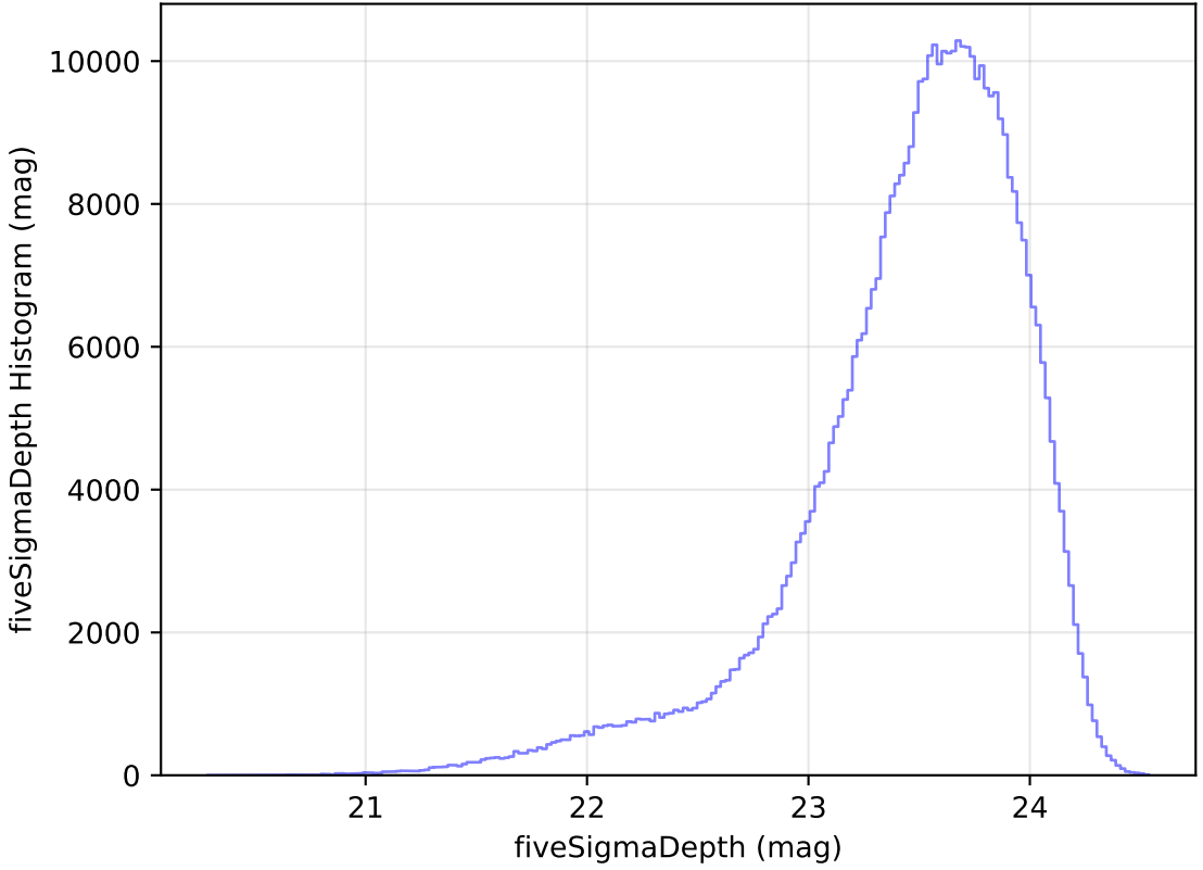
too_elab_r16_d3_ugrizy_v3.4_10yrs WFD i band: fiveSigmaDepth Histogram
