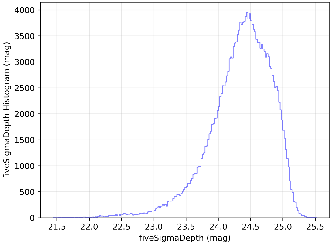
too_elab_r16_d3_ugrizy_v3.4_10yrs WFD g band: fiveSigmaDepth Histogram
