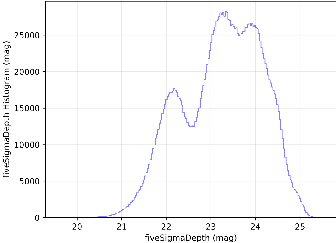
too_elab_r16_d3_ugrizy_v3.4_10yrs WFD all bands: fiveSigmaDepth Histogram
