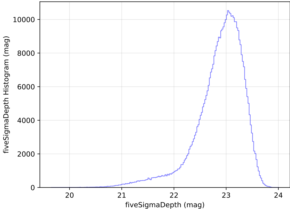
too_elab_r16_d3_ugrizy_v3.4_10yrs All sky z band: fiveSigmaDepth Histogram
