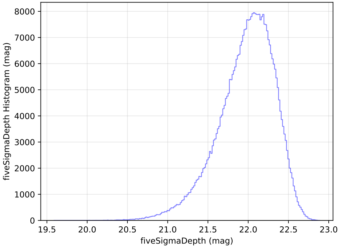
too_elab_r16_d3_ugrizy_v3.4_10yrs All sky y band: fiveSigmaDepth Histogram
