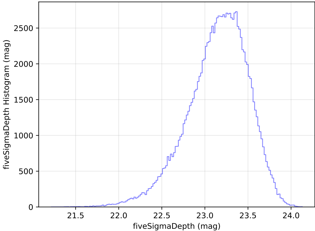
too_elab_r16_d3_ugrizy_v3.4_10yrs All sky u band: fiveSigmaDepth Histogram
