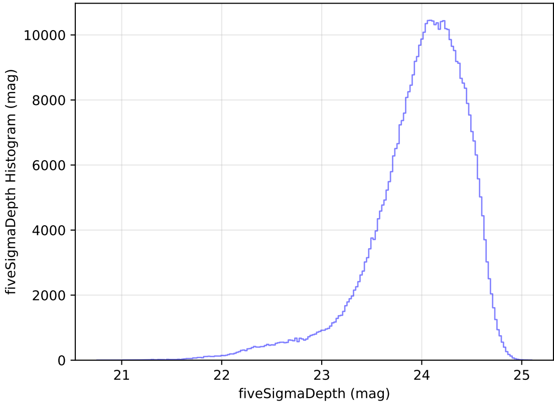
too_elab_r16_d3_ugrizy_v3.4_10yrs All sky r band: fiveSigmaDepth Histogram
