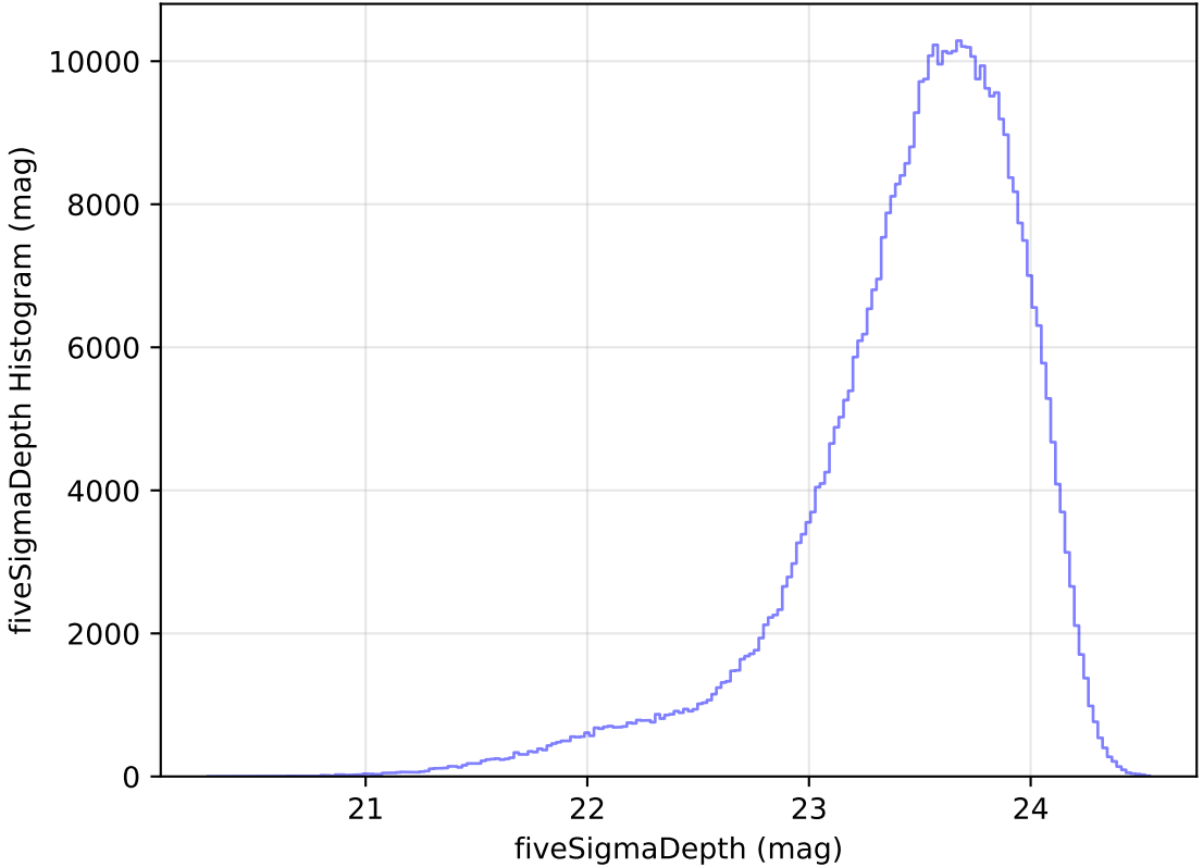
too_elab_r16_d3_ugrizy_v3.4_10yrs All sky i band: fiveSigmaDepth Histogram
