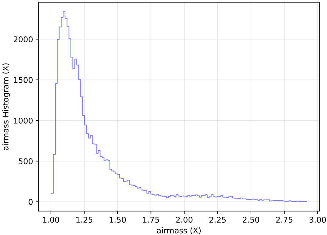
too_elab_r16_d3_ugrizy_v3.4_10yrs Yr 1 z band: airmass Histogram
