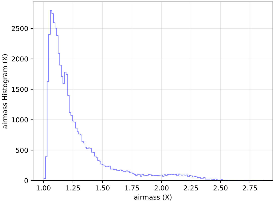
too_elab_r16_d3_ugrizy_v3.4_10yrs Yr 1 r band: airmass Histogram
