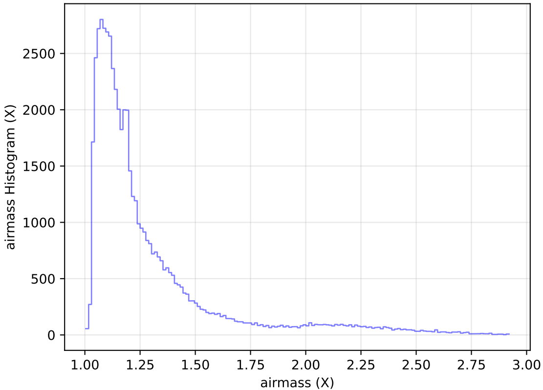
too_elab_r16_d3_ugrizy_v3.4_10yrs Yr 1 i band: airmass Histogram
