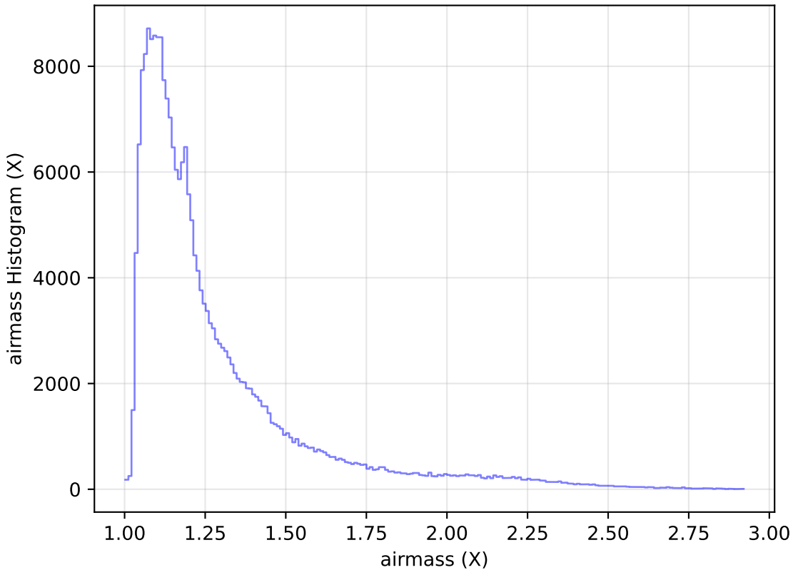
too_elab_r16_d3_ugrizy_v3.4_10yrs Yr 1 all bands: airmass Histogram
