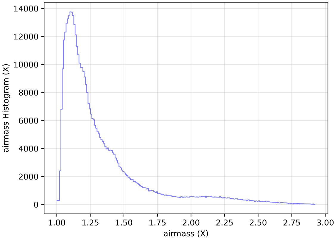
too_elab_r16_d3_ugrizy_v3.4_10yrs WFD z band: airmass Histogram
