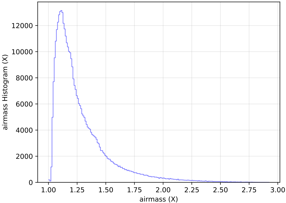
too_elab_r16_d3_ugrizy_v3.4_10yrs WFD y band: airmass Histogram
