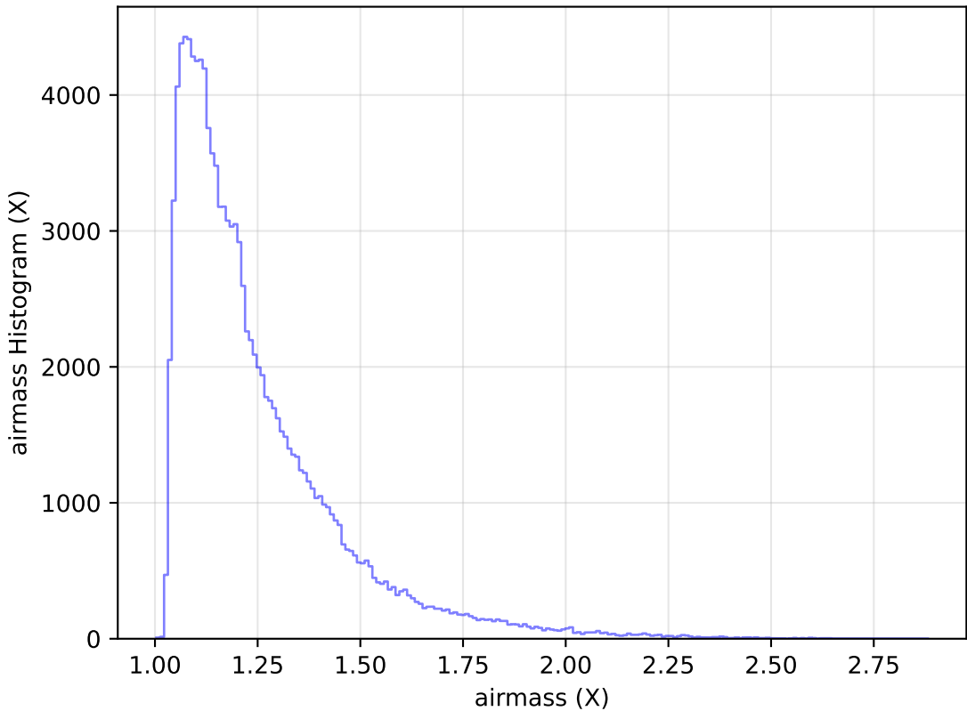
too_elab_r16_d3_ugrizy_v3.4_10yrs WFD u band: airmass Histogram
