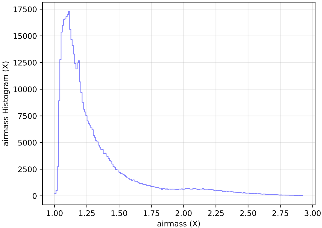
too_elab_r16_d3_ugrizy_v3.4_10yrs WFD i band: airmass Histogram
