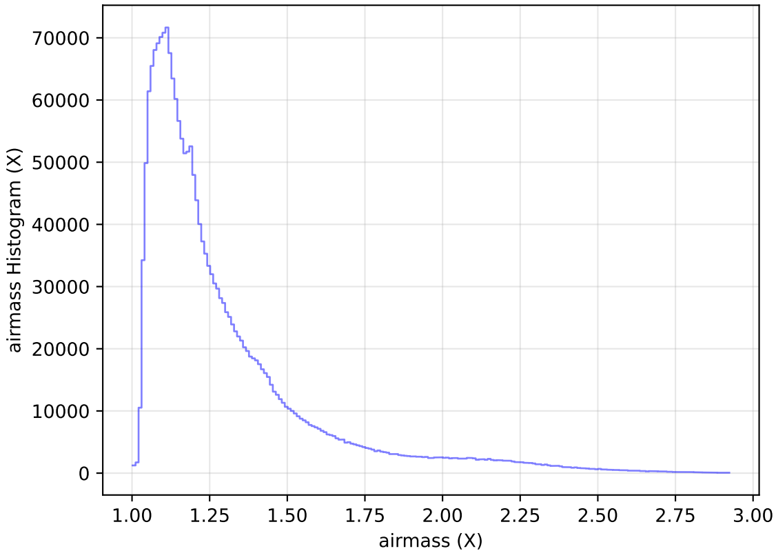
too_elab_r16_d3_ugrizy_v3.4_10yrs WFD all bands: airmass Histogram
