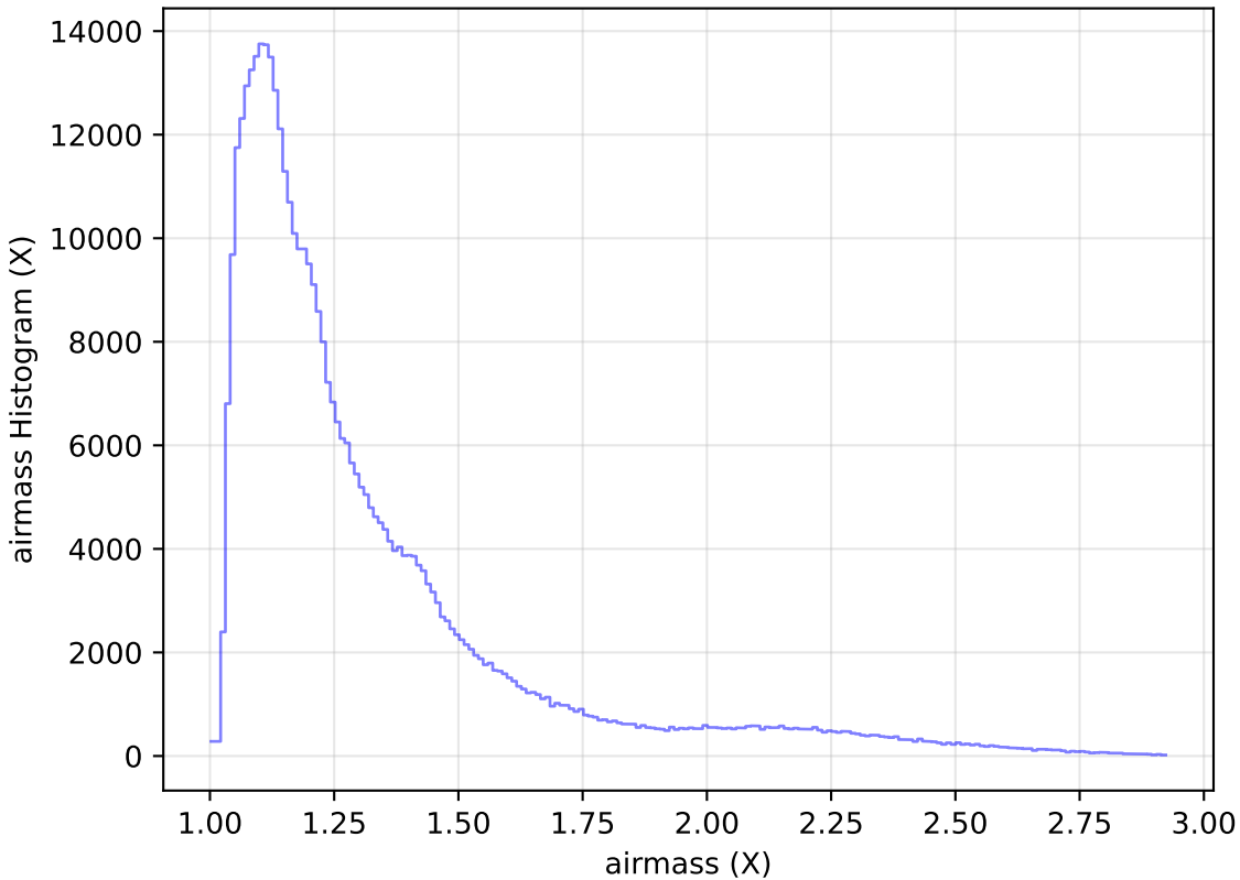
too_elab_r16_d3_ugrizy_v3.4_10yrs All sky z band: airmass Histogram
