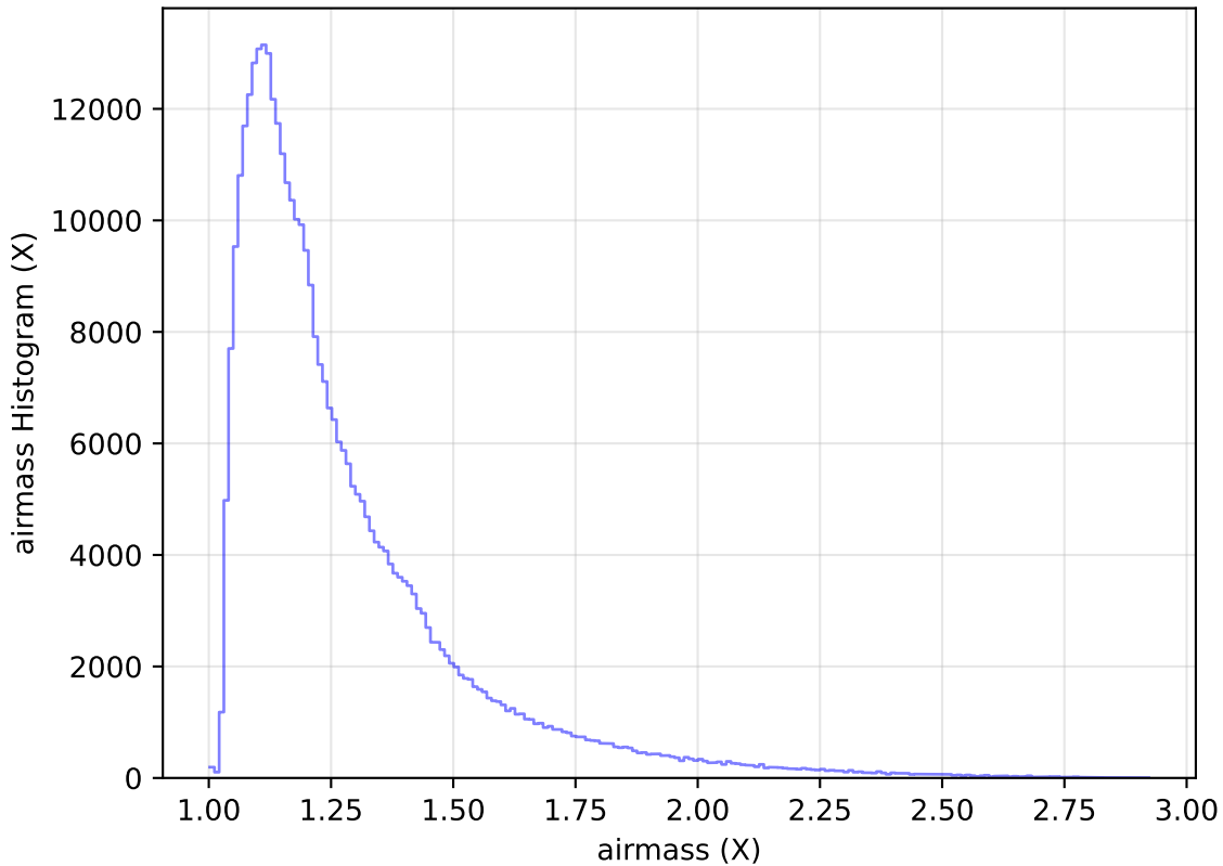
too_elab_r16_d3_ugrizy_v3.4_10yrs All sky y band: airmass Histogram
