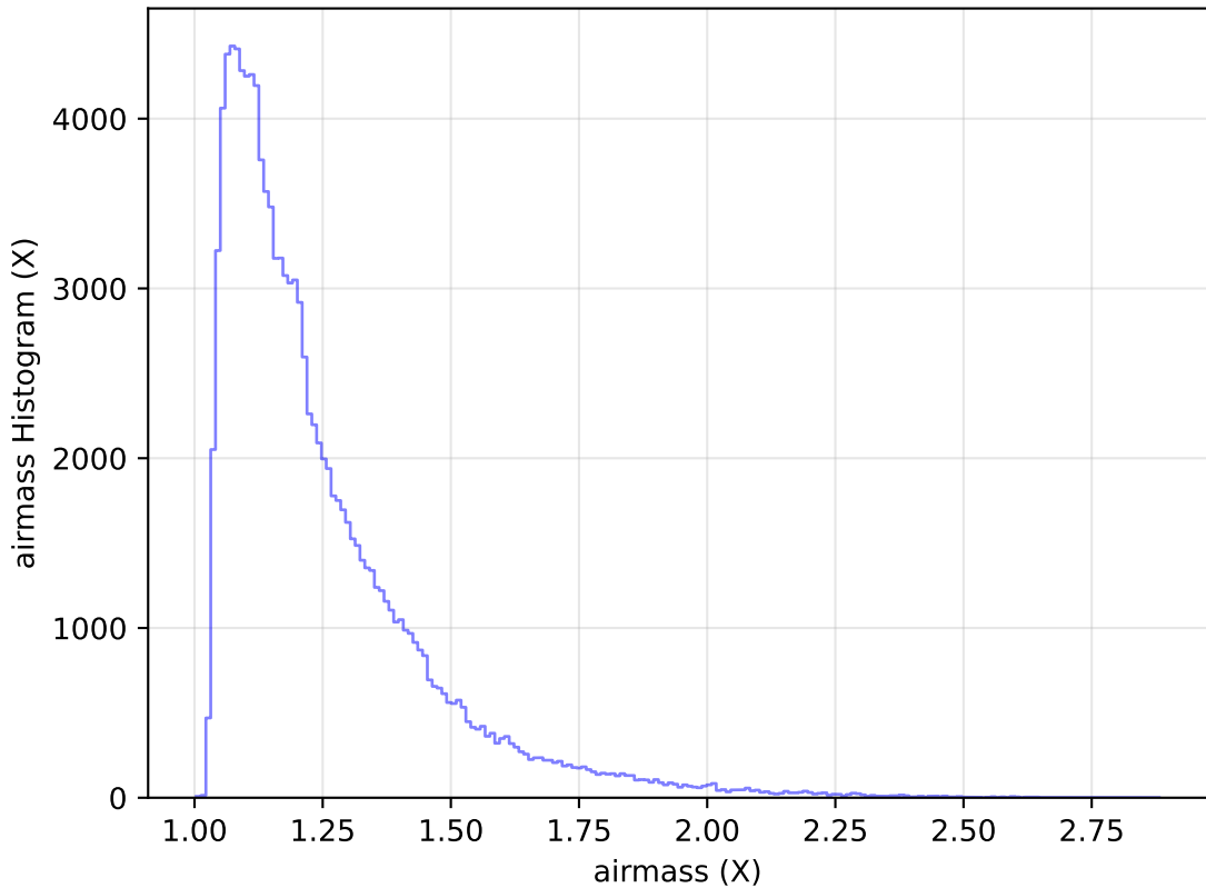
too_elab_r16_d3_ugrizy_v3.4_10yrs All sky u band: airmass Histogram
