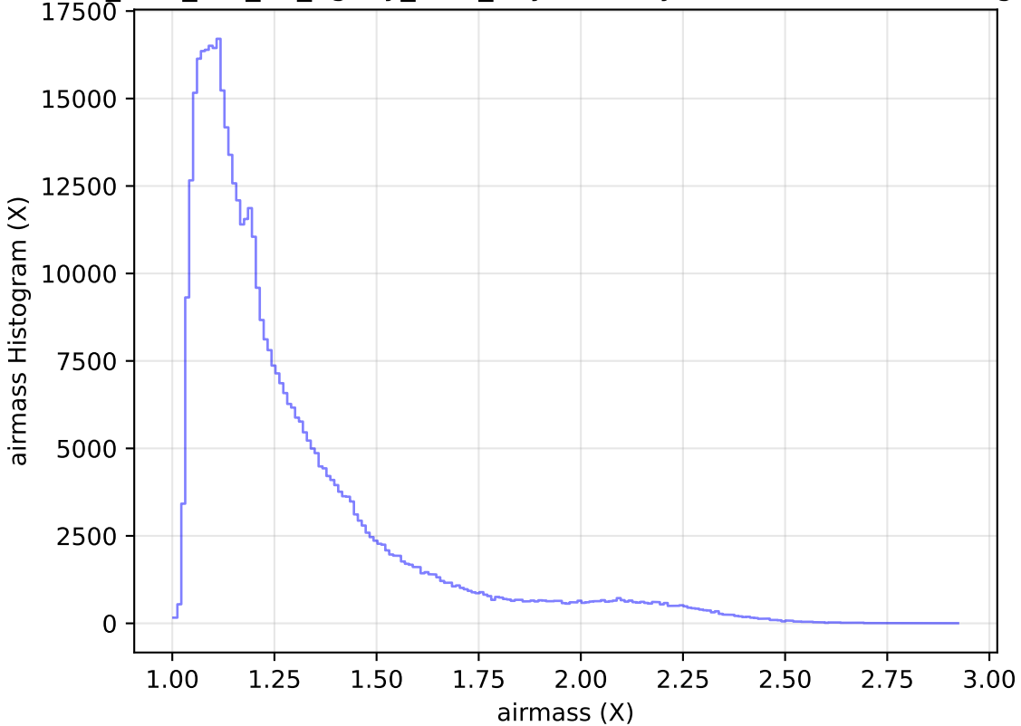
too_elab_r16_d3_ugrizy_v3.4_10yrs All sky r band: airmass Histogram
