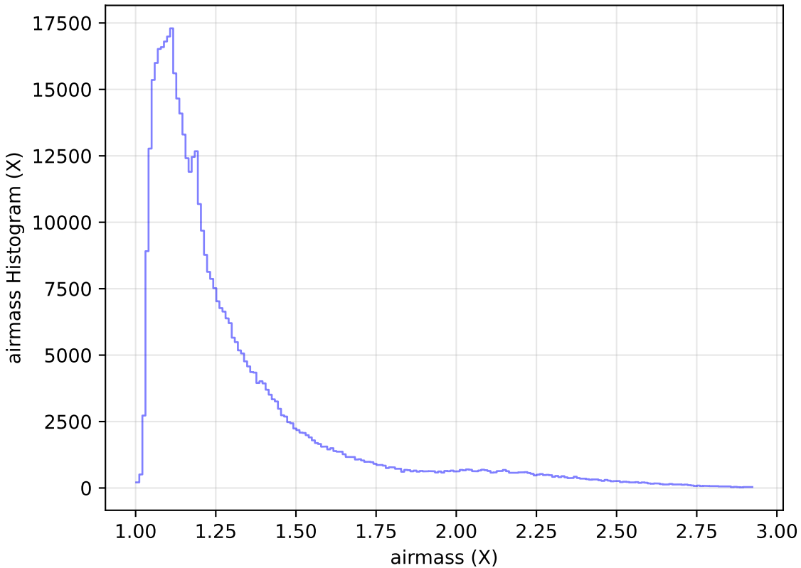
too_elab_r16_d3_ugrizy_v3.4_10yrs All sky i band: airmass Histogram
