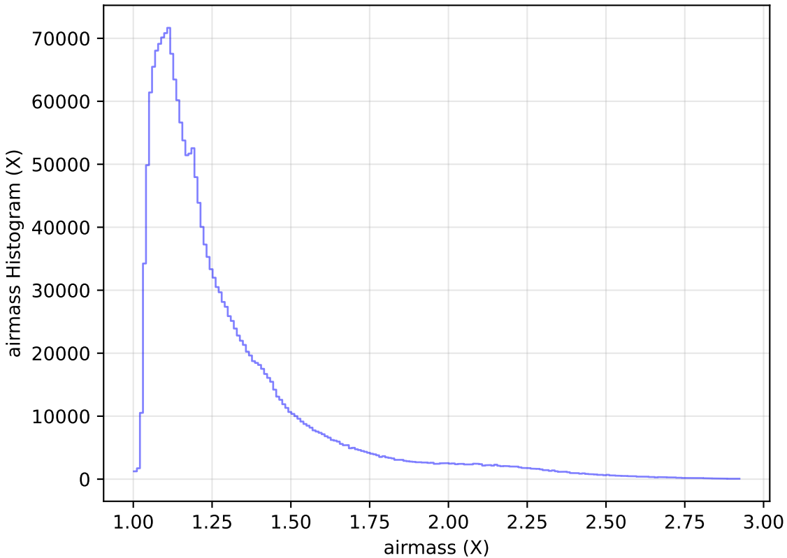
too_elab_r16_d3_ugrizy_v3.4_10yrs All sky all bands: airmass Histogram
