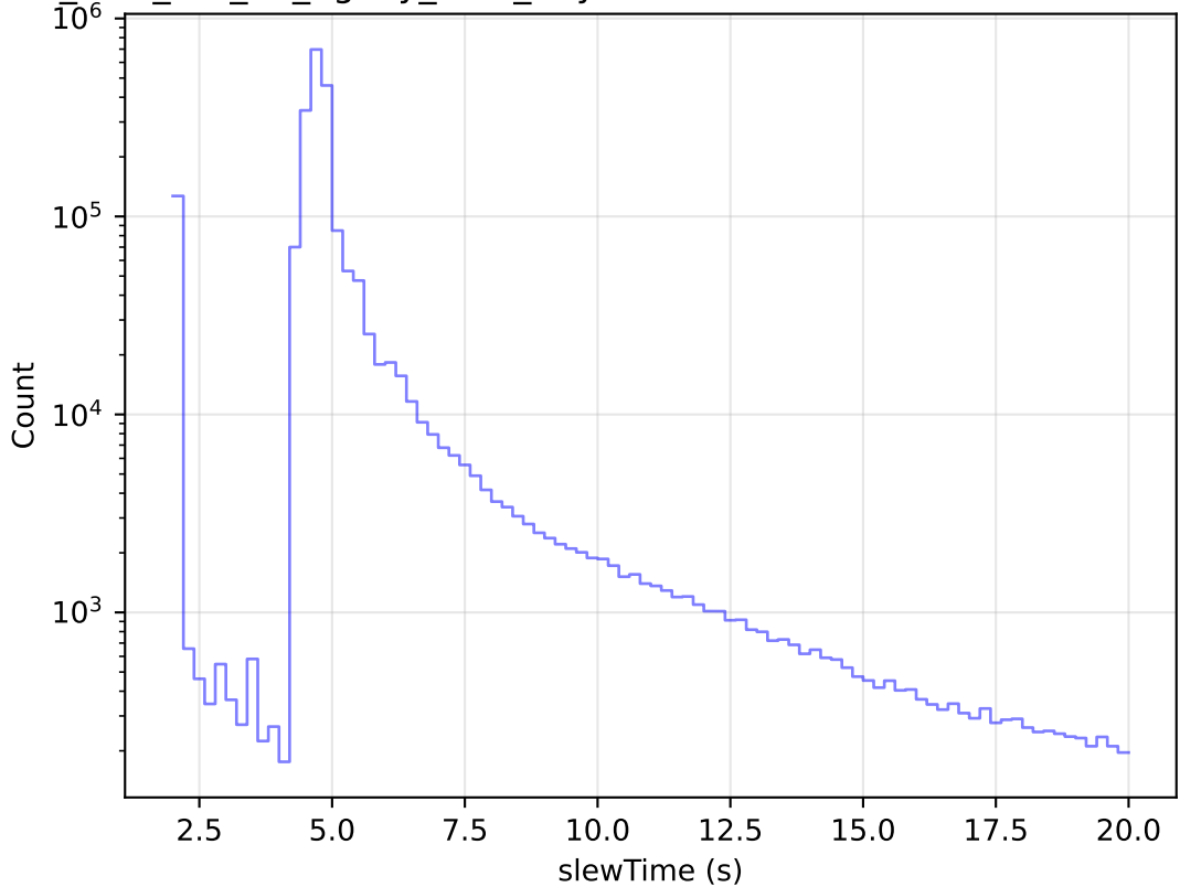
too_elab_r16_d3_ugrizy_v3.4_10yrs All visits: Zoom Slew Time Histogram
