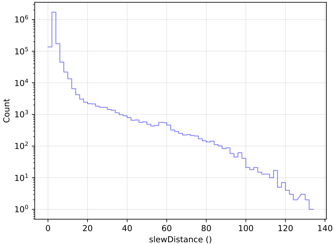
too_elab_r16_d3_ugrizy_v3.4_10yrs All visits: Slew Distance Histogram
