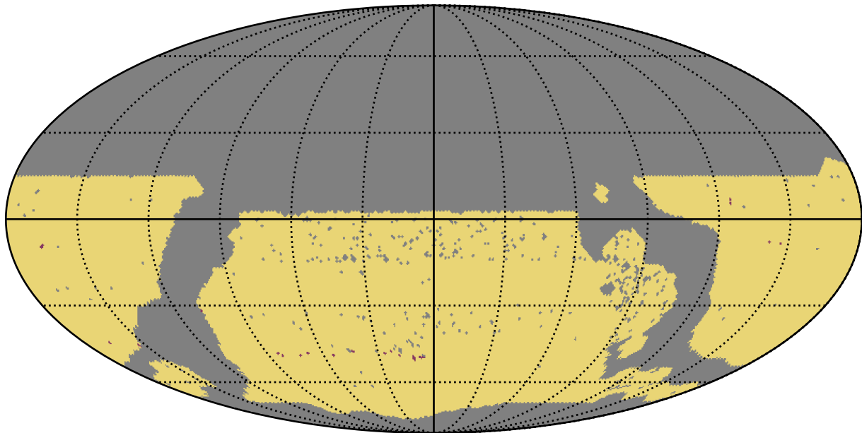
too_elab_r16_d3_ugrizy_v3.4_10yrs WFD: RapidRevisits
