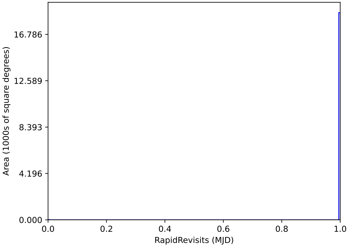
too_elab_r16_d3_ugrizy_v3.4_10yrs WFD: RapidRevisits
