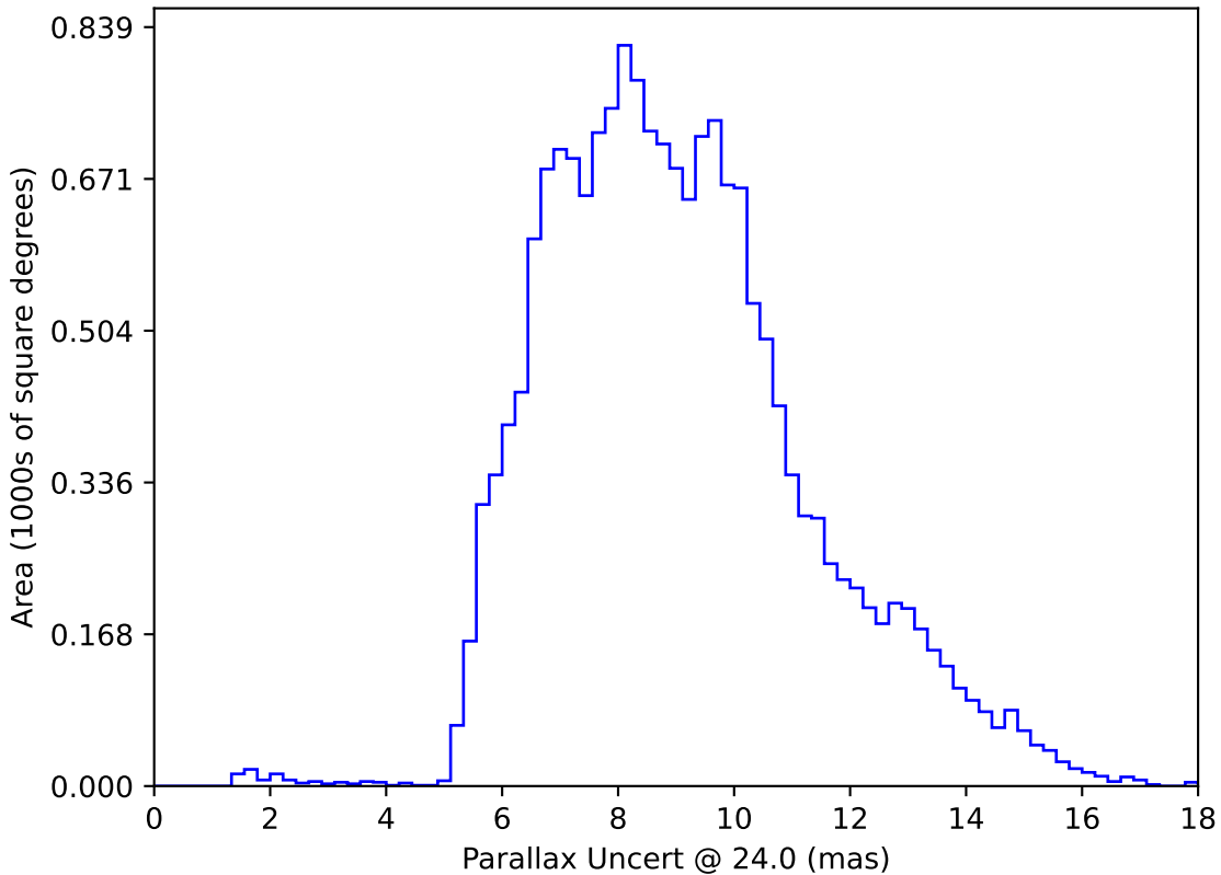
too_elab_r16_d3_ugrizy_v3.4_10yrs WFD: Parallax Uncert @ 24.0
