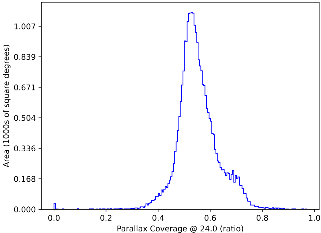
too_elab_r16_d3_ugrizy_v3.4_10yrs All sky: Parallax Coverage @ 24.0
