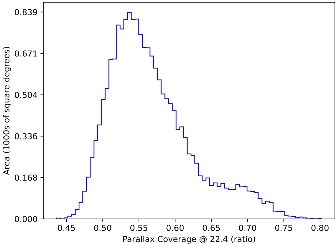
too_elab_r16_d3_ugrizy_v3.4_10yrs WFD: Parallax Coverage @ 22.4
