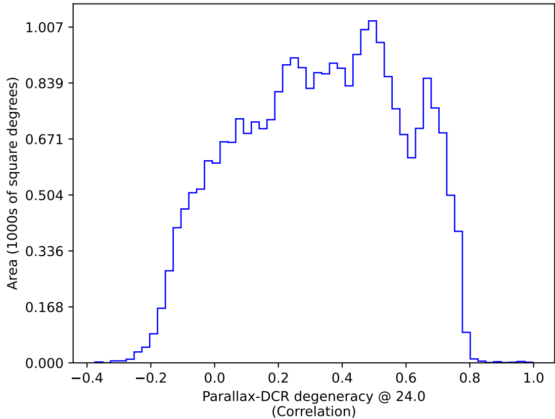
too_elab_r16_d3_ugrizy_v3.4_10yrs All sky: Parallax-DCR degeneracy @ 24.0
