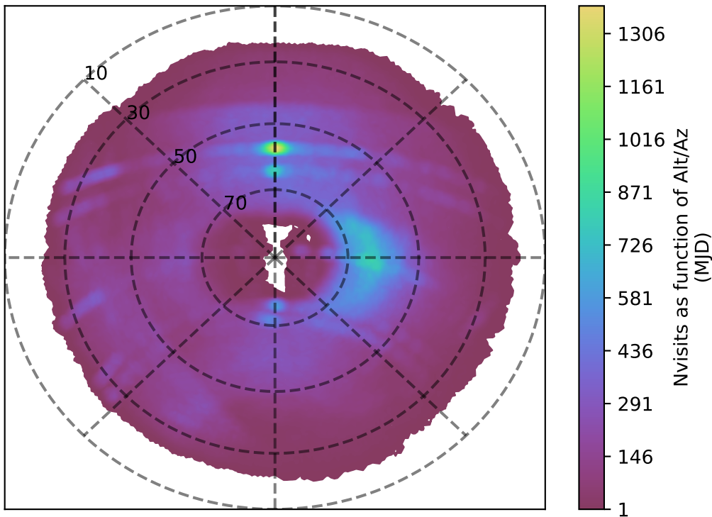
too_elab_r16_d3_ugrizy_v3.4_10yrs g band: Nvisits as function of Alt/Az
