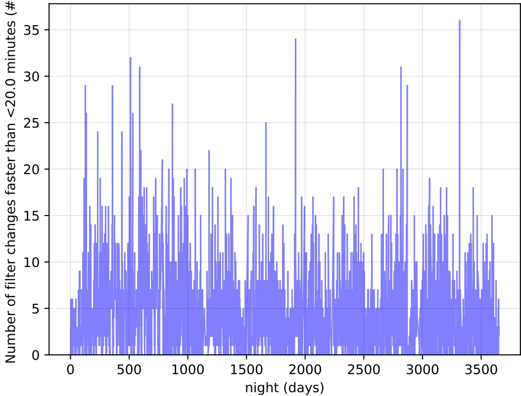
too_elab_r16_d3_ugrizy_v3.4_10yrs Per Night: Number of filter changes faster than <20.0 minutes
