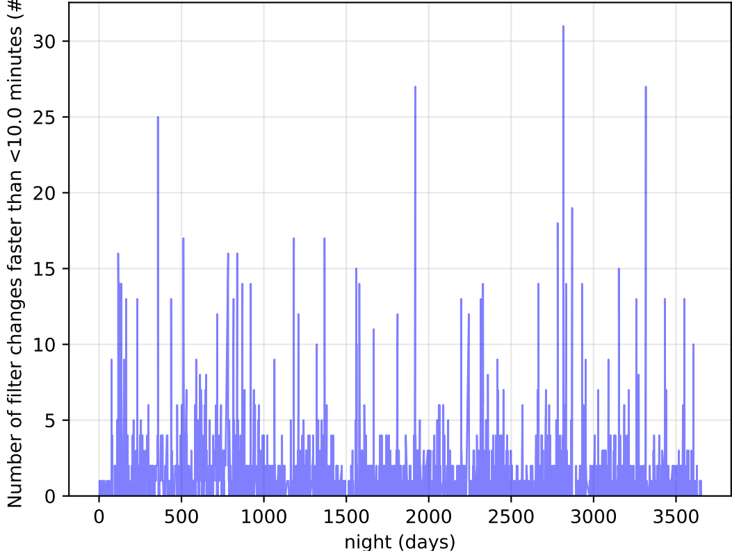
too_elab_r16_d3_ugrizy_v3.4_10yrs Per Night: Number of filter changes faster than <10.0 minutes
