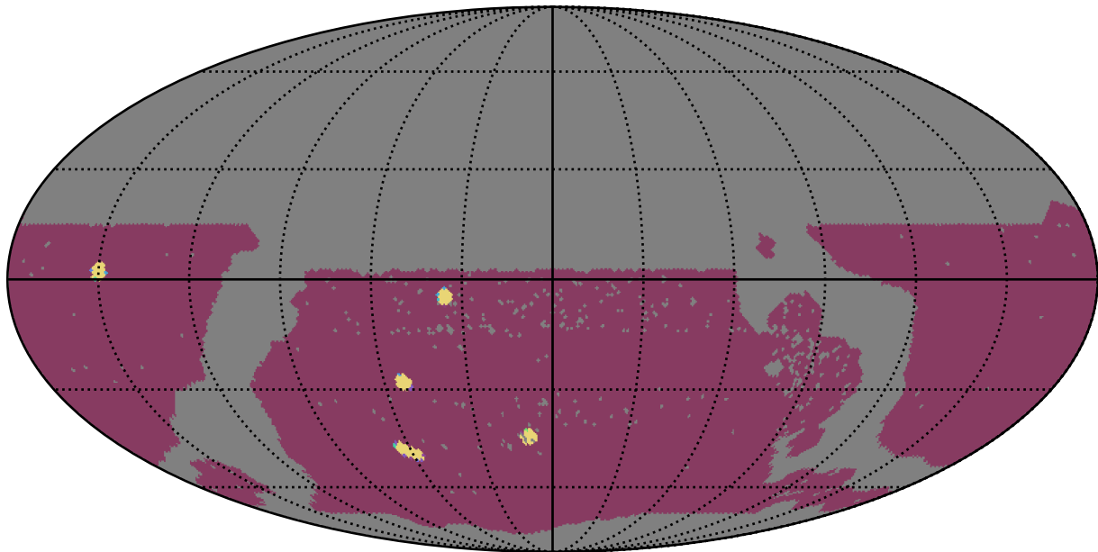
too_elab_r16_d3_ugrizy_v3.4_10yrs WFD: NumberOfQuickRevisits
