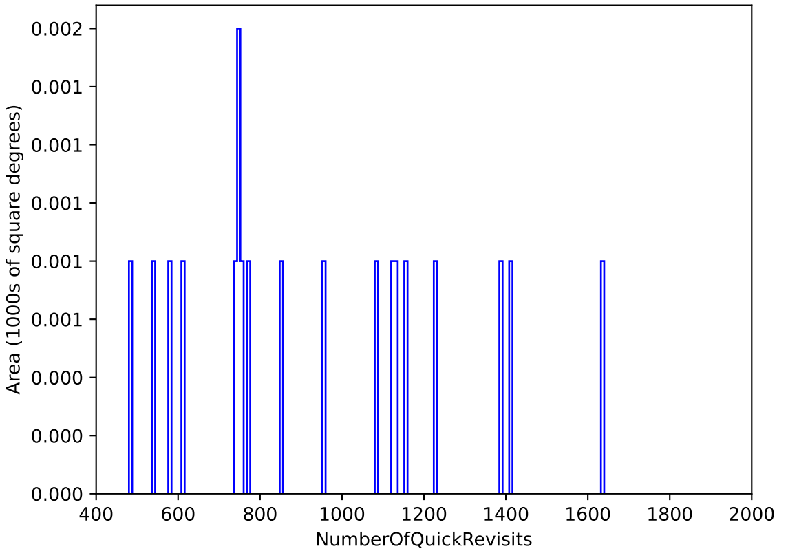
too_elab_r16_d3_ugrizy_v3.4_10yrs WFD: NumberOfQuickRevisits
