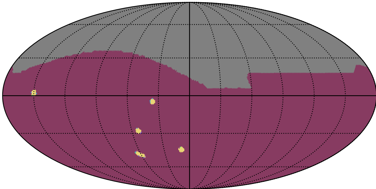
too_elab_r16_d3_ugrizy_v3.4_10yrs All sky: NumberOfQuickRevisits
